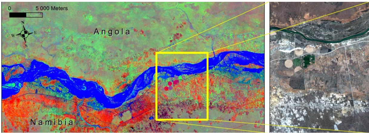
Figure 1: Landsat-based Spectral Mixture Analysis for 2010 (left, RGB = Bare ground, Vegetation, Water) and corresponding Quickbird subset (right, RGB = 3-2-1)
