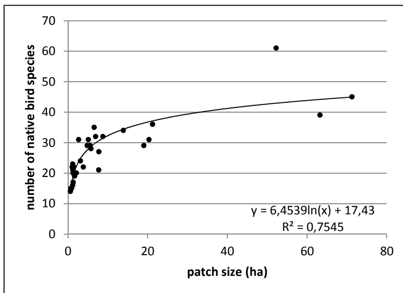
Figure 2: Number of native bird species in relation to size of green spaces.
