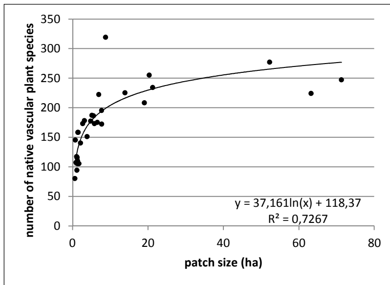
Figure 1: Number of native vascular plant species in relation to size of green spaces.
